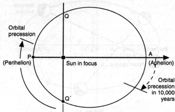
Figure 11 ADVANCE OF THE PERIHELION OR ORBITAL PRECESSION
